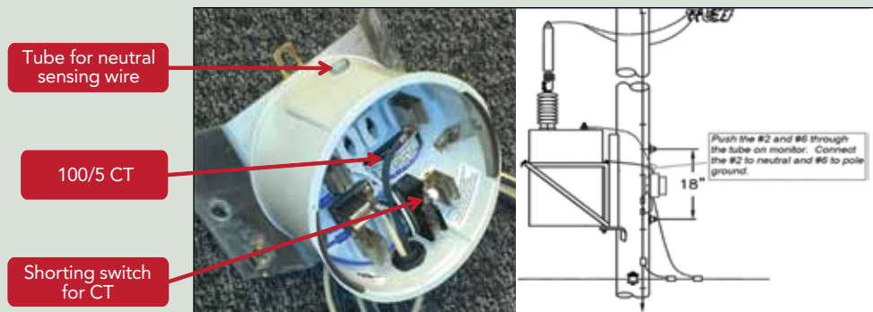
A view of the adapter without the AMI meter installed.
