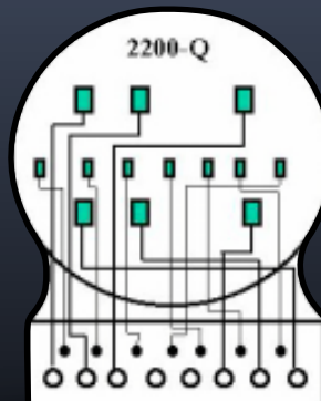
CT Meter Form 8S
