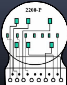
CT Meter Form 9S
