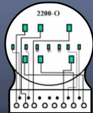
CT Meter Form 6S
