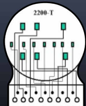
CT Meter Form 9S
