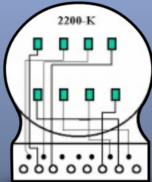
CT Meter Form 5S
