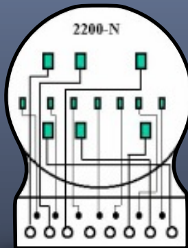
CT Meter Forms 6S, 9S, 10S
