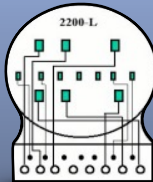
CT Meter Form 6S
