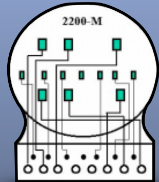
CT Meter Form 10S
